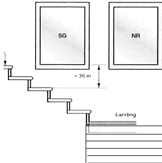
Section view
